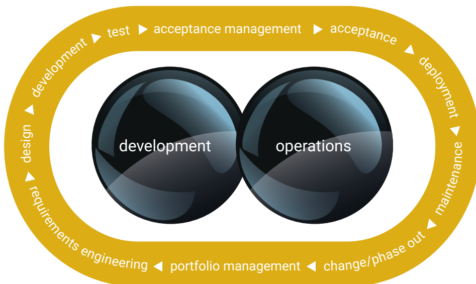
Figure 1: Application Lifecycle
